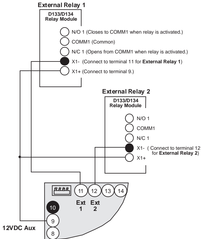
Figure 4: External Relay Wiring
