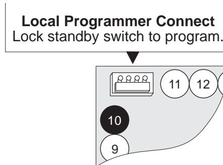
Figure 9: Programmer Jack
