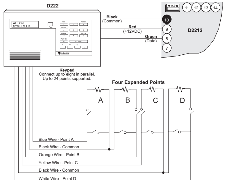
Figure 3: Keypad Wiring
